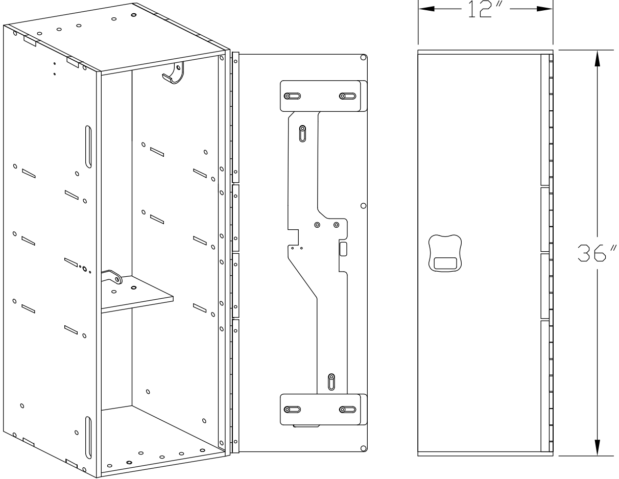
ISOMETRIC VIEW
