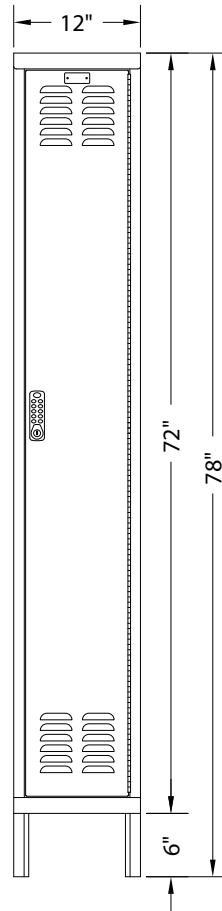
FRONT VIEW
