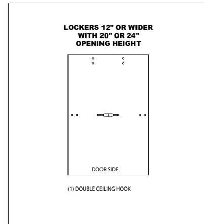
HOOK CONFIGURATION
