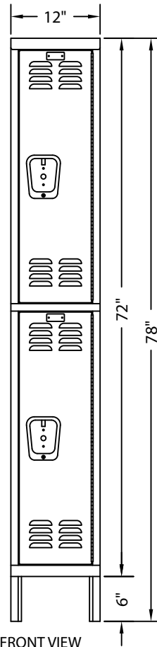
FRONT VIEW
