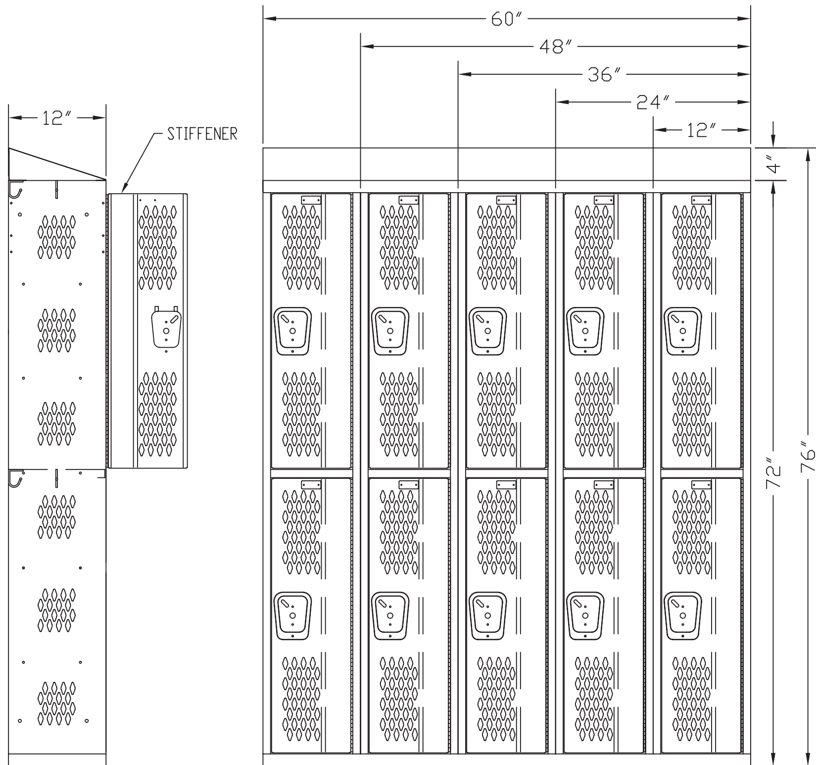
SIDE VIEW
