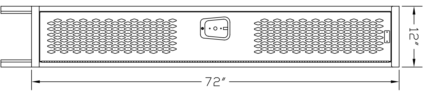
FRONT VIEW 1-WIDE
