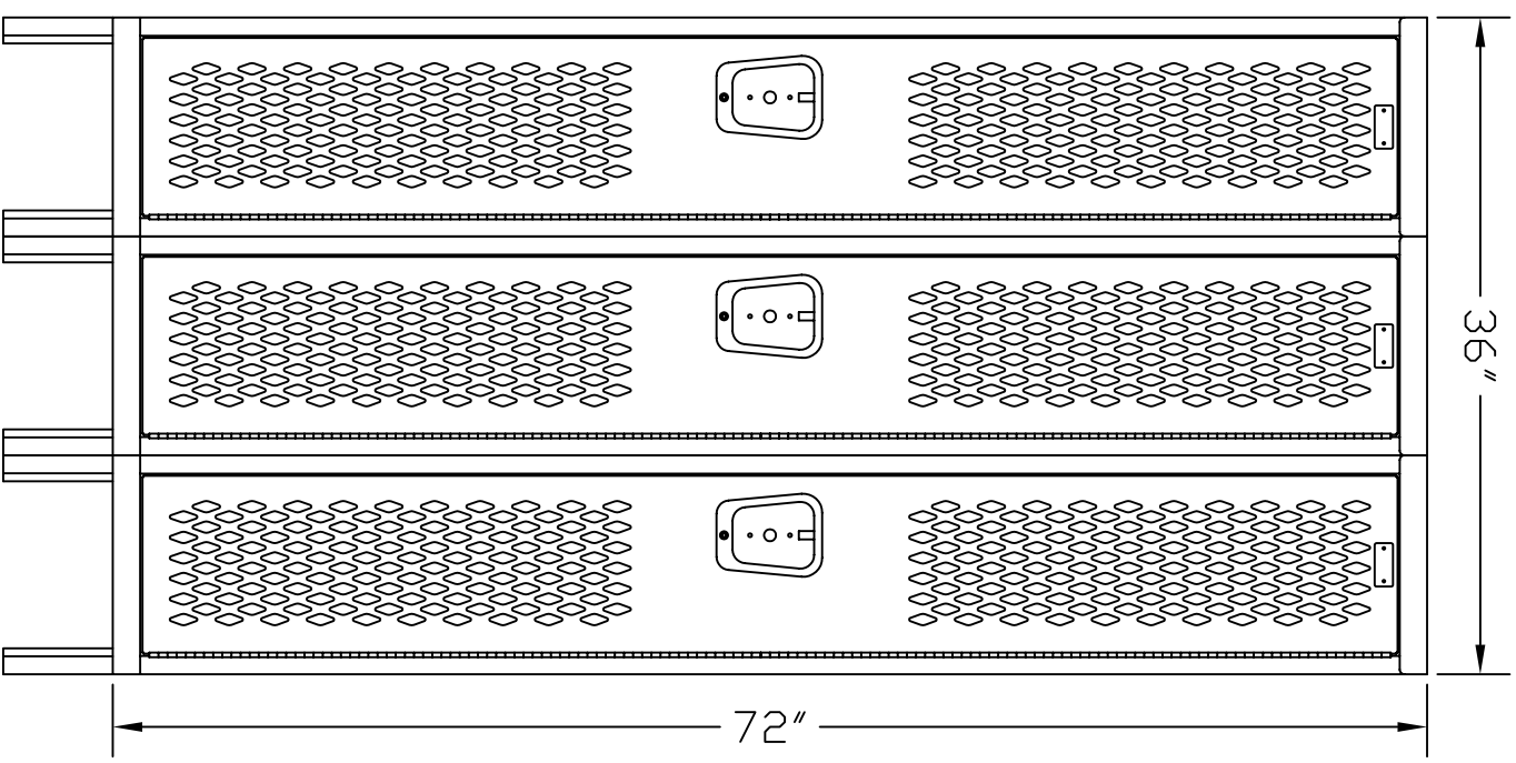
FRONT VIEW 3-WIDE
