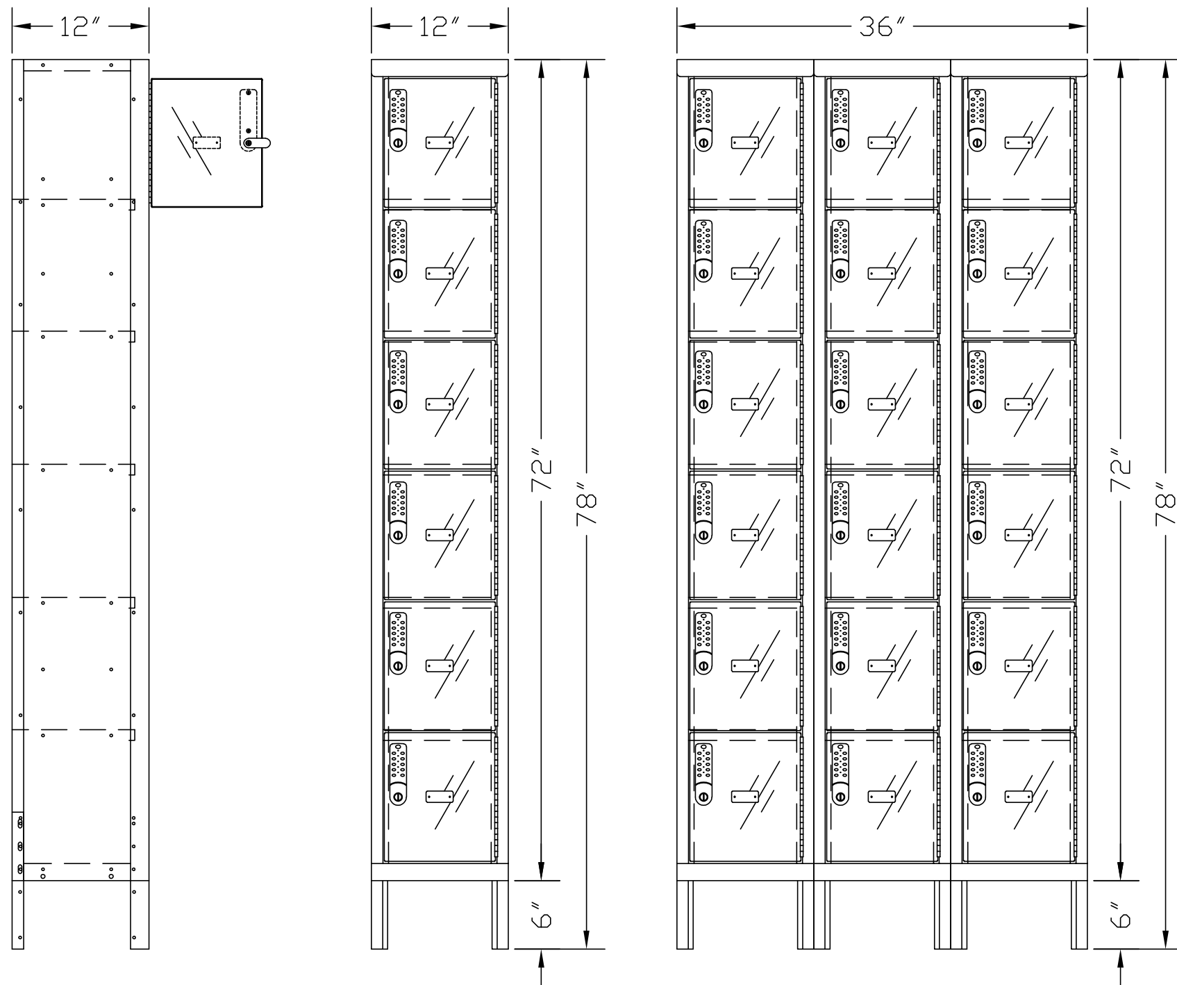
SIDE VIEW
