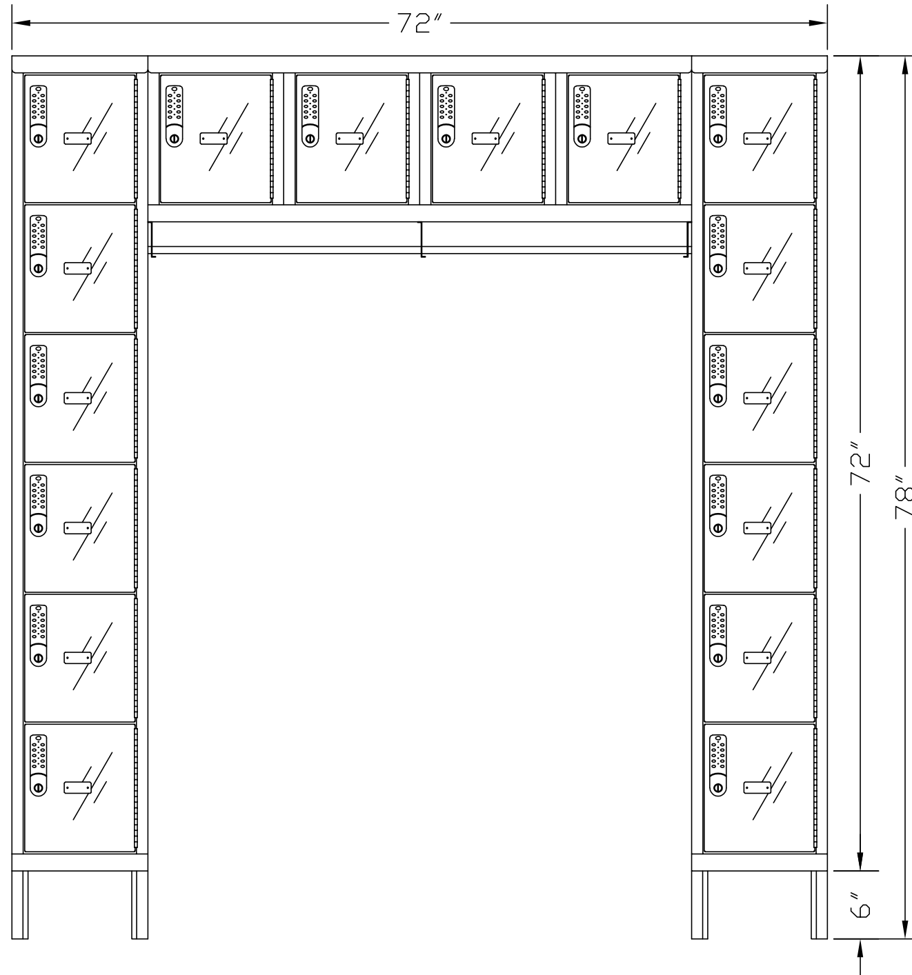
FRONT VIEW
