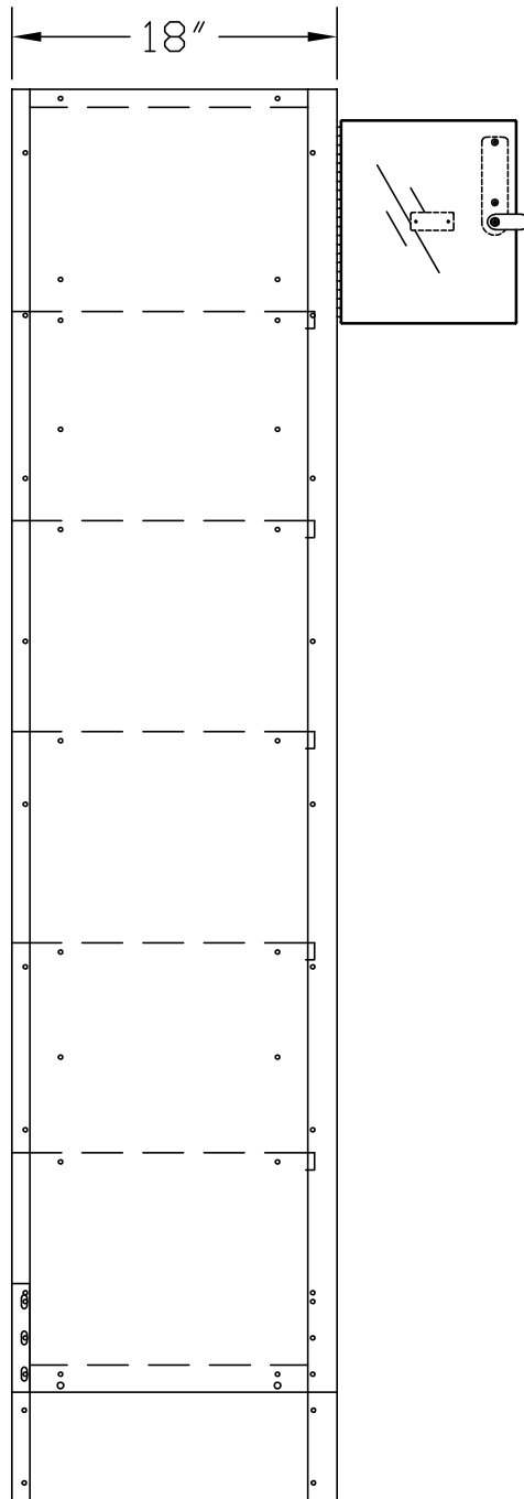
SIDE VIEW
