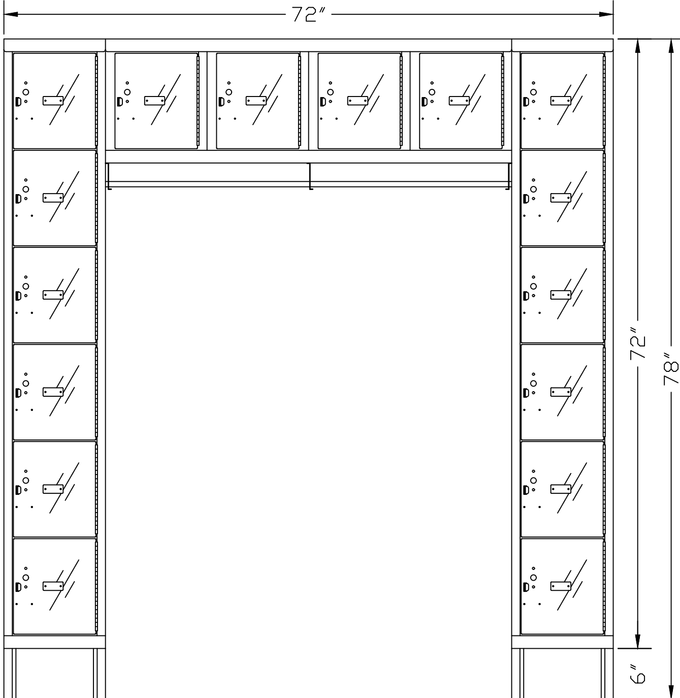
FRONT VIEW
